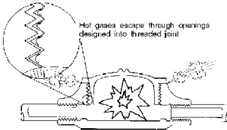
OPENINGS DESIGNED INTO THREADED JOINT
